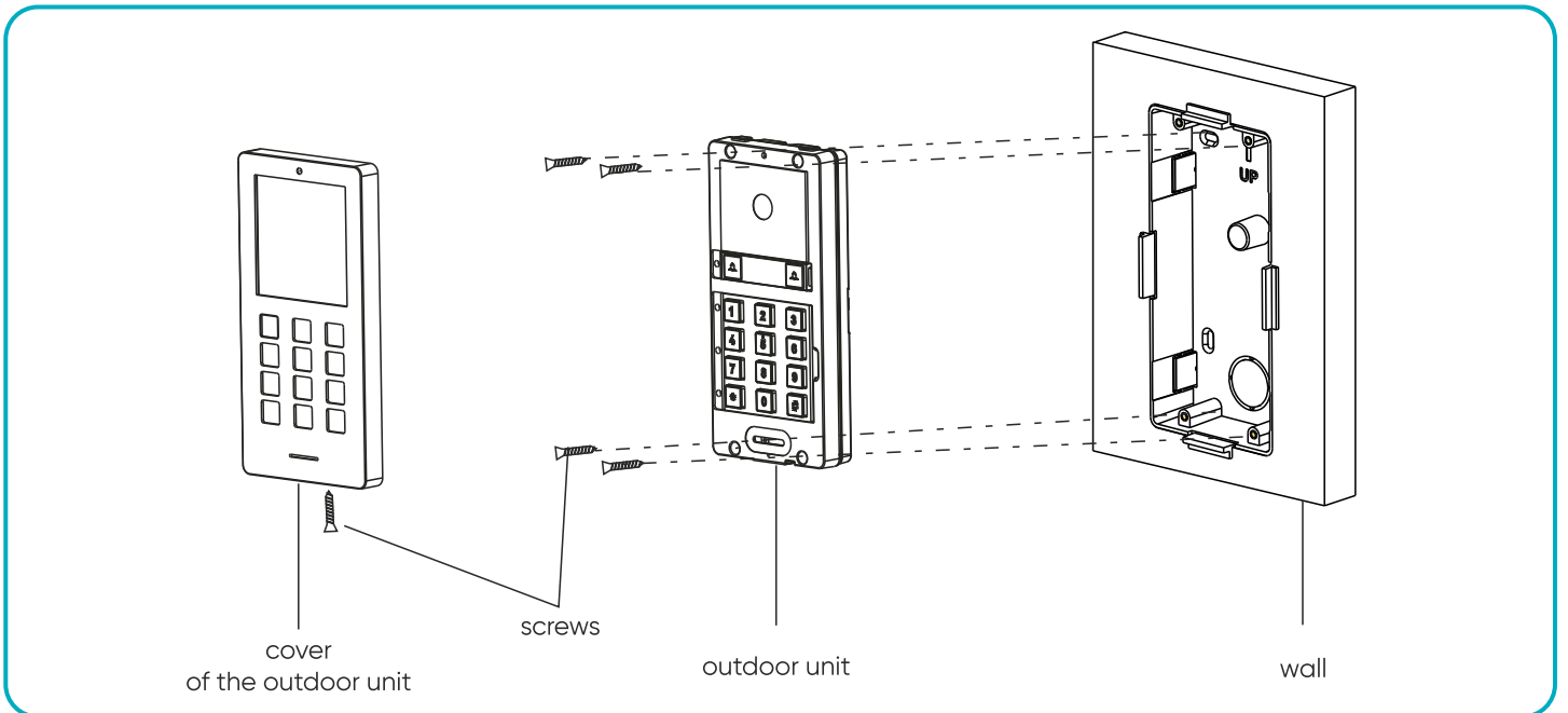
fig. 6 Outdoor unit with camera flush installation.
