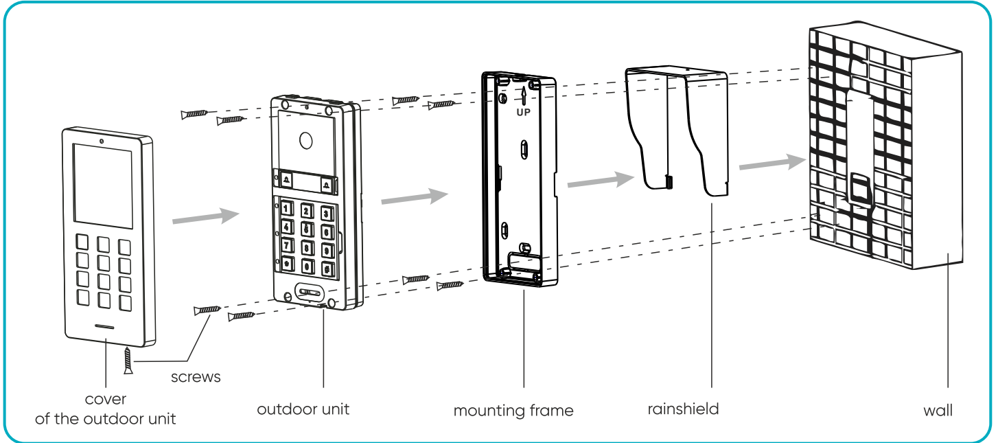
fig. 5 Outdoor unit with camera surface installation.
