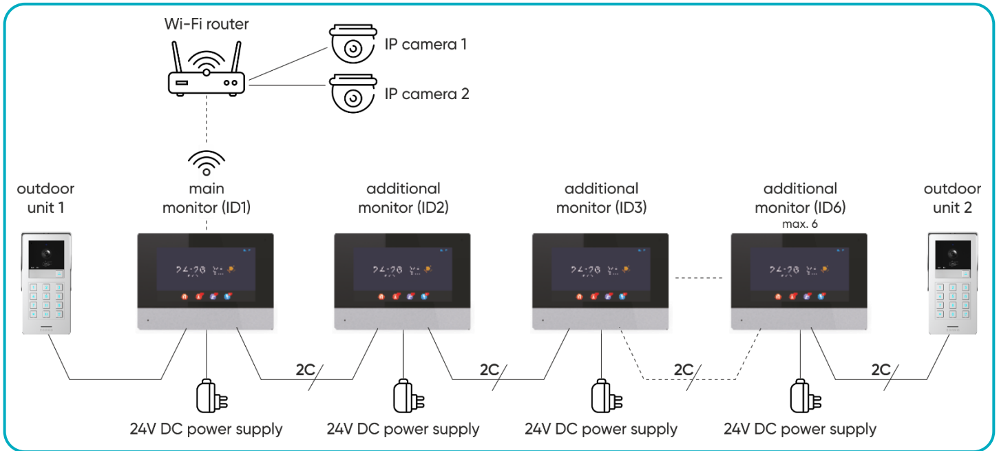
fig. 7 Single-family set wiring diagram.
