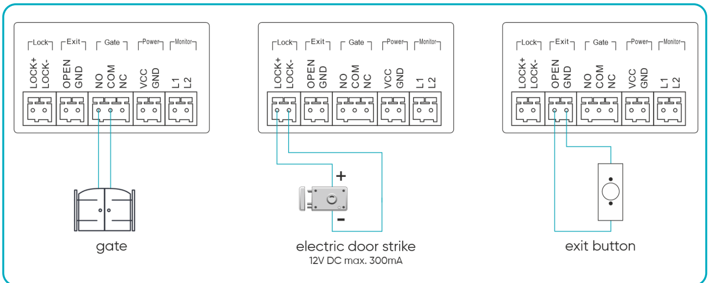
fig. 12 Gate, electric door strike, and exit button wiring scheme.
