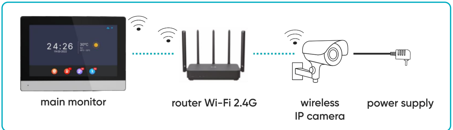
fig. 14 Connection scheme for the monitor and wireless IP camera.
