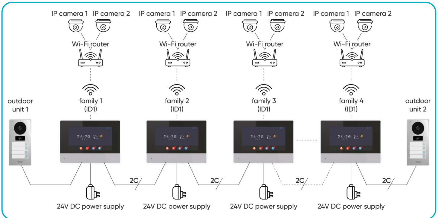
fig. 9 Four-family set wiring diagram.
