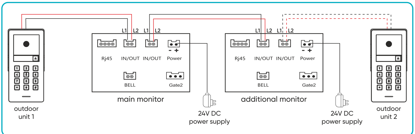
fig. 10 Monitors and outdoor units wiring diagram.
