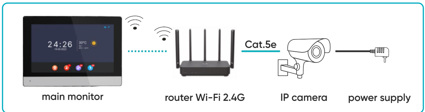
fig. 13 Connection scheme for the monitor and wired IP camera.
