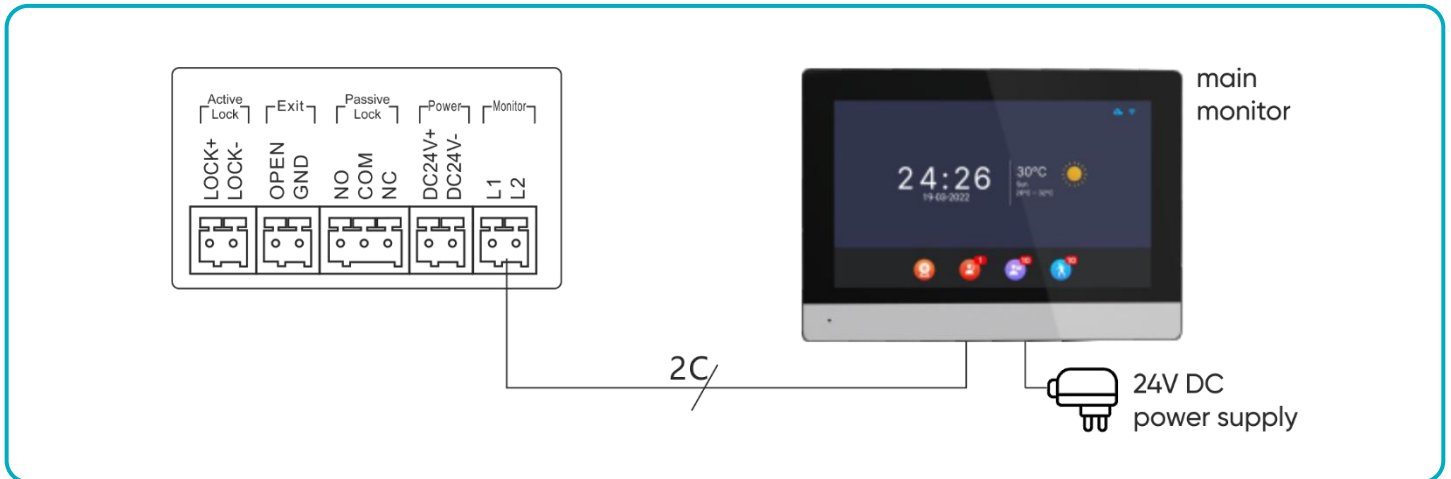
fig. 11 Monitor and outdoor unit wiring diagram.
