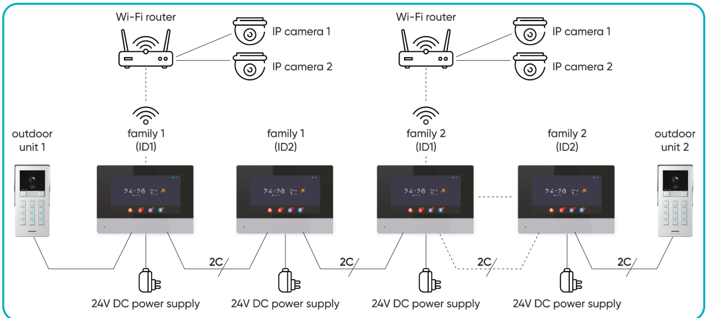
fig. 8 Two-family set wiring diagram.
